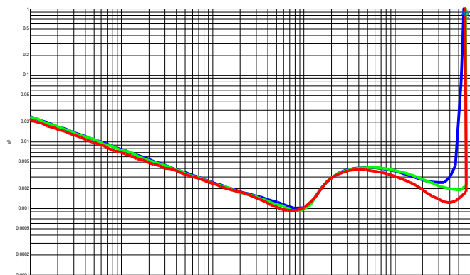
THD+N vs. power at 100Hz (blue), 1kHz (green) and 6kHz (red) (2Ω).
