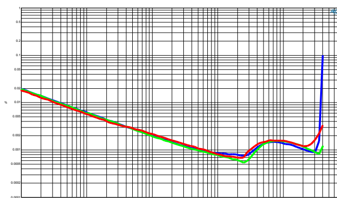
THD+N vs. power at 100Hz (blue), 1kHz (green) and 6kHz (red) (4Ω).
