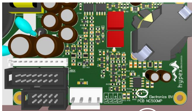
Figure 1 Placement of the bypass resistors
