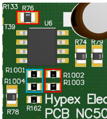
Figure 2 Resistors in the red squares need to be removed, resistors in the blue square need to be added for unbuffered operation
