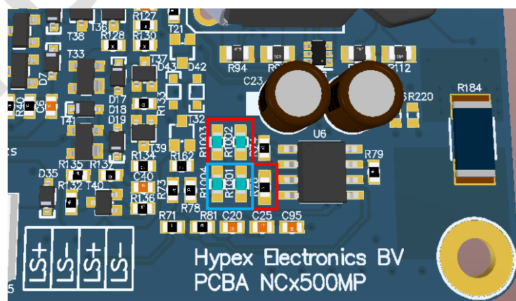
Figure 2 Resistors in the red squares need to be removed, resistors in the blue square need to be added for unbuffered operation
