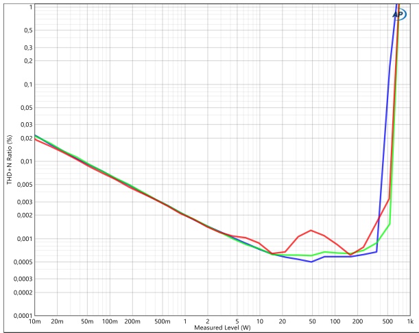
THD+N vs. power at 100Hz (blue), 1kHz (green) and 6kHz (red) (2Ω).
