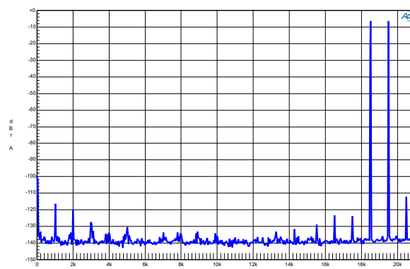
IMD spectrum at 18.5kHz + 19.5kHz, P_R/2 in 4Ω (blue).
