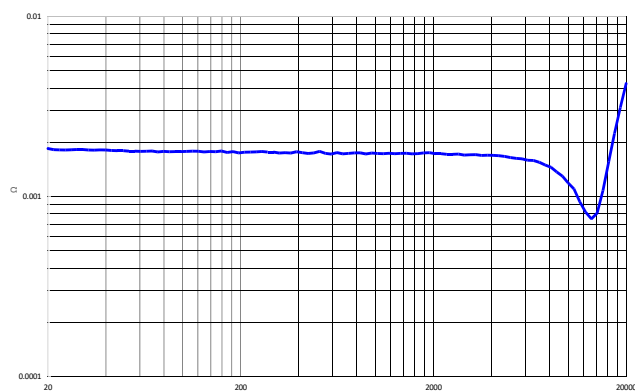
Output impedance
