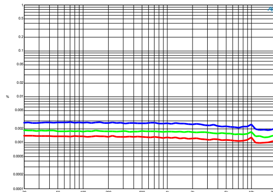
THD+N vs. Frequency at 1W in 2Ω (blue), 4Ω (green) and 8Ω (red).
