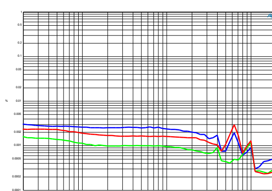
THD+N vs. Frequency at P_R/2 in 2Ω (blue), 4Ω (green) and 8Ω (red).
