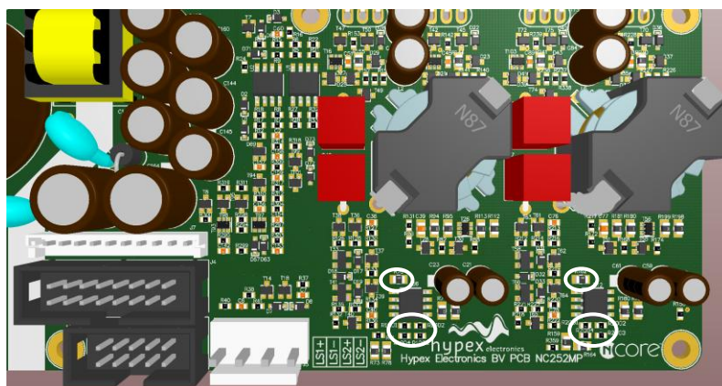
Figure 1 Placement of the bypass resistors
