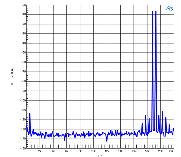
IMD spectrum at 18.5kHz + 19.5kHz, P_R/2 in 4Ω (blue).
