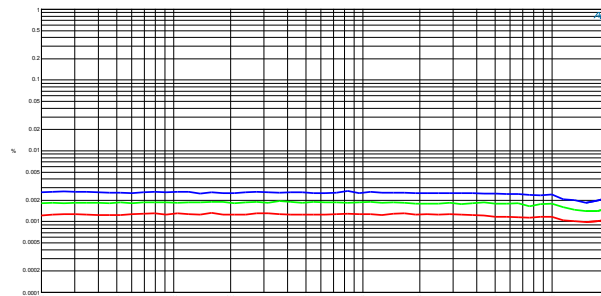
THD+N vs. Frequency at 1W in 2Ω (blue), 4Ω (green) and 8Ω (red).
