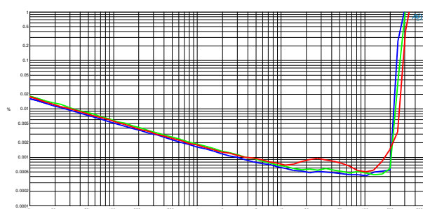
THD+N vs. power at 100Hz (blue), 1kHz (green) and 6kHz (red) (4Ω).
