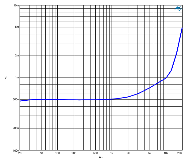
Output impedance
