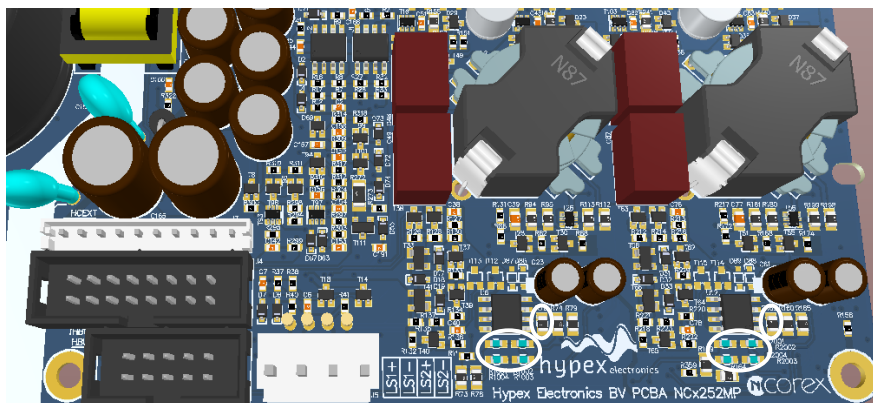
Figure 1 Placement of the bypass resistors
