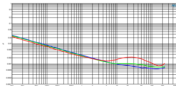
THD+N vs. power at 100Hz (blue), 1kHz (green) and 6kHz (red) (2Ω).
