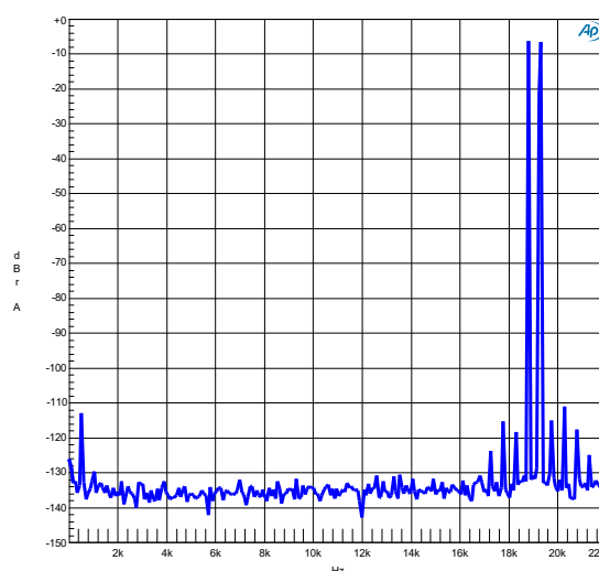
IMD spectrum at 18.5kHz + 19.5kHz, P_R/2 in 4Ω (blue).
