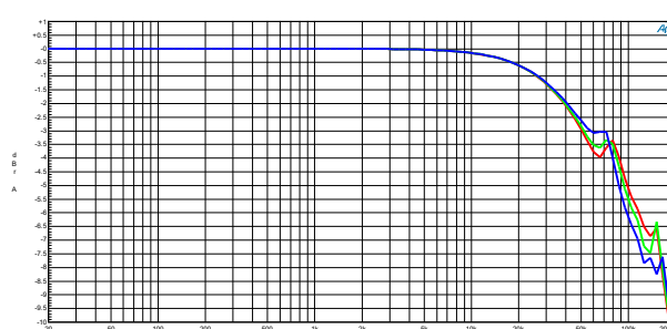
Frequency response in 2Ω (blue), 4Ω (green) and 8Ω (red).
