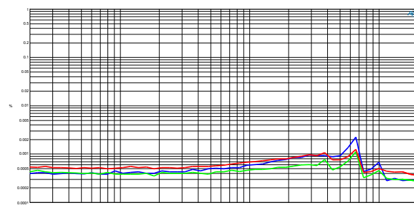
THD+N vs. Frequency at P_R/2 in 2Ω (blue), 4Ω (green) and 8Ω (red).
