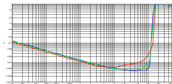
THD+N vs. power at 100Hz (blue), 1kHz (green) and 6kHz (red) (8Ω).
