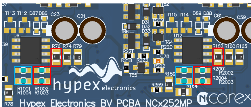
Figure 2 Resistors in the red squares need to be removed, resistors in the blue squares need to be added for unbuffered operation
