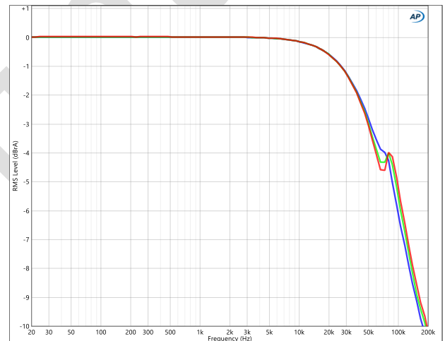
Frequency response in 2Ω (blue), 4Ω (green) and 8Ω (red).
