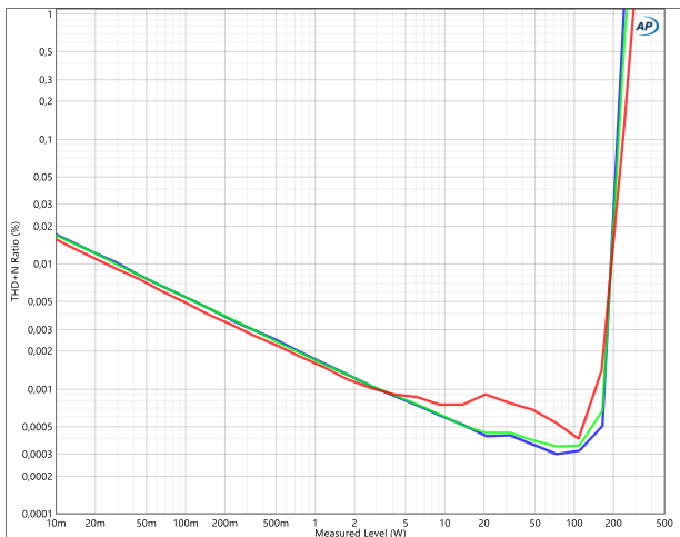
THD+N vs. power at 100Hz (blue), 1kHz (green) and 6kHz (red) (4Ω).
