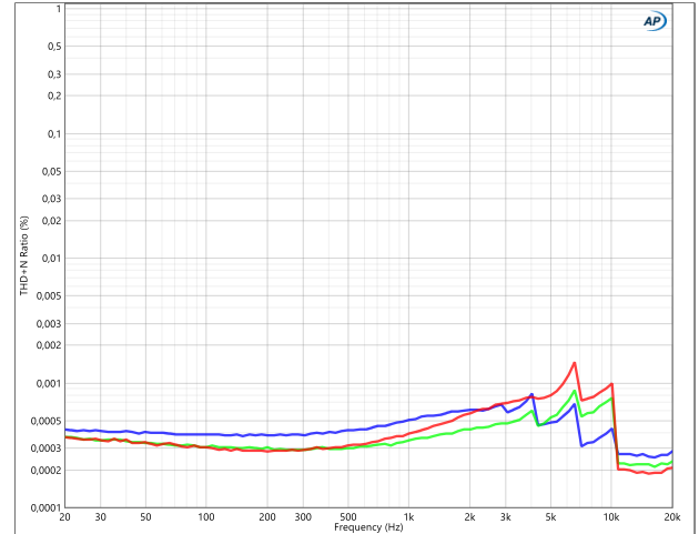
THD+N vs. Frequency at P_R/2 in 2Ω (blue), 4Ω (green) and 8Ω (red).
