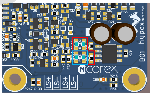
Figure 2 Resistors in the red squares need to be removed, resistors in the blue square need to be added for unbuffered operation
