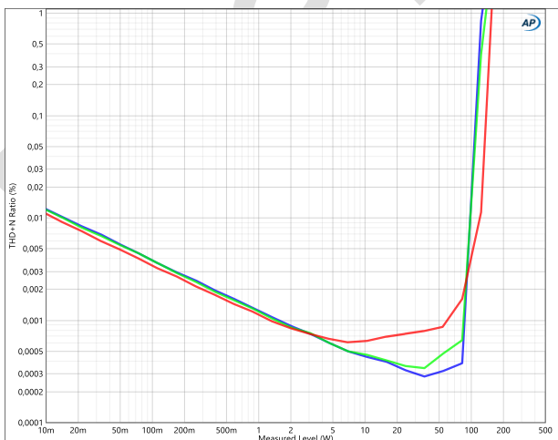
THD+N vs. power at 100Hz (blue), 1kHz (green) and 6kHz (red) (8Ω).
