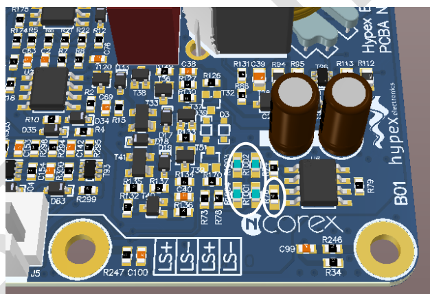
Figure 1 Placement of the bypass resistors
