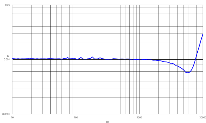
Output impedance
