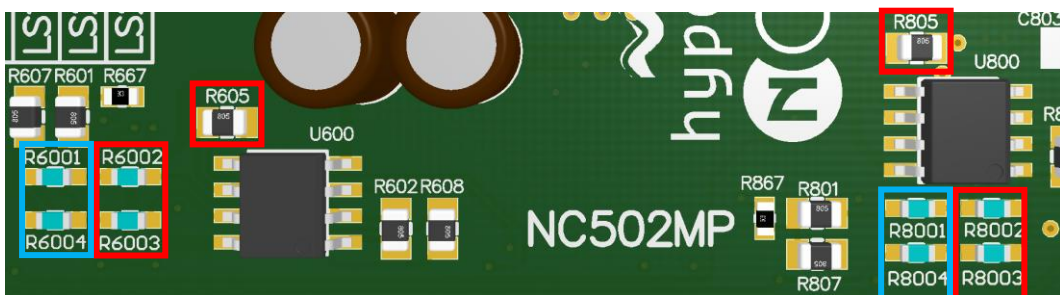
Figure 2 Resistors in the red squares need to be removed, resistors in the blue squares need to be added for unbuffered operation
