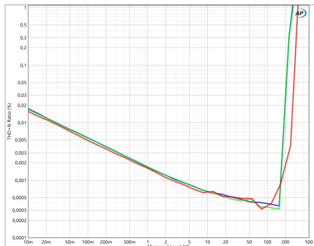
THD+N vs. power at 100Hz (blue), 1kHz (green) and 6kHz (red) (BTL - 8 \Omega ).
