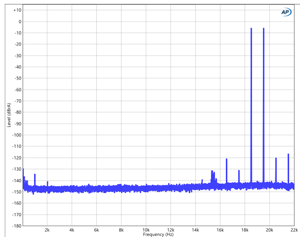
IMD spectrum at 18.5kHz + 19.5kHz, P_R/2 in 4Ω (blue).
