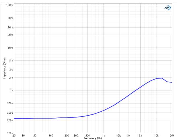
Output impedance
