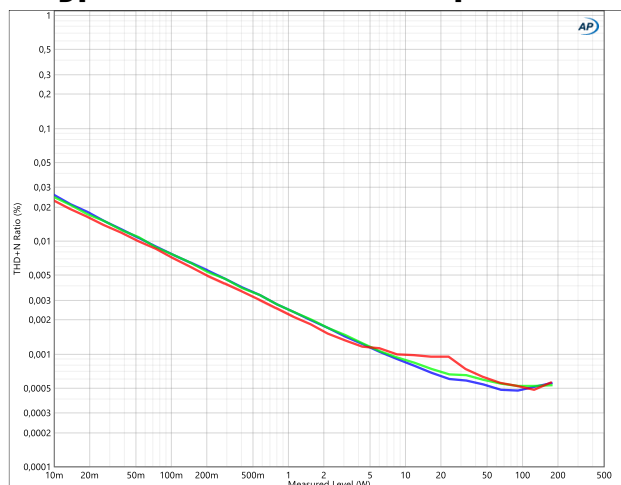
THD+N vs. power at 100Hz (blue), 1kHz (green) and 6kHz (red) (BTL - 4 \Omega ).
