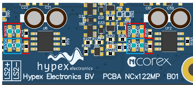
Figure 2 Resistors in the red squares need to be removed, resistors in the blue squares need to be added for unbuffered operation
